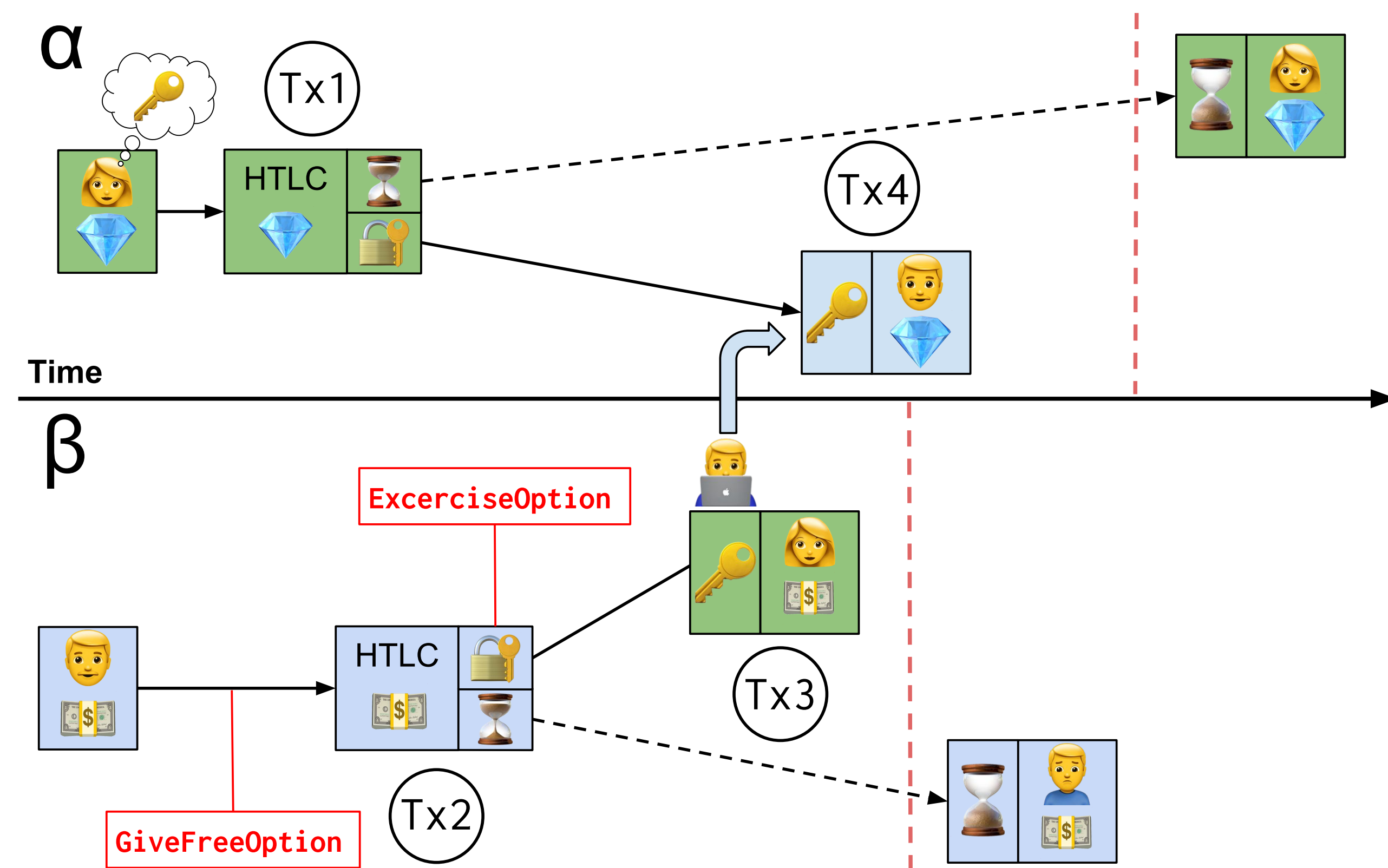
Figure 1: Atomic Swap Protocol - by Tier Nolan [3]
