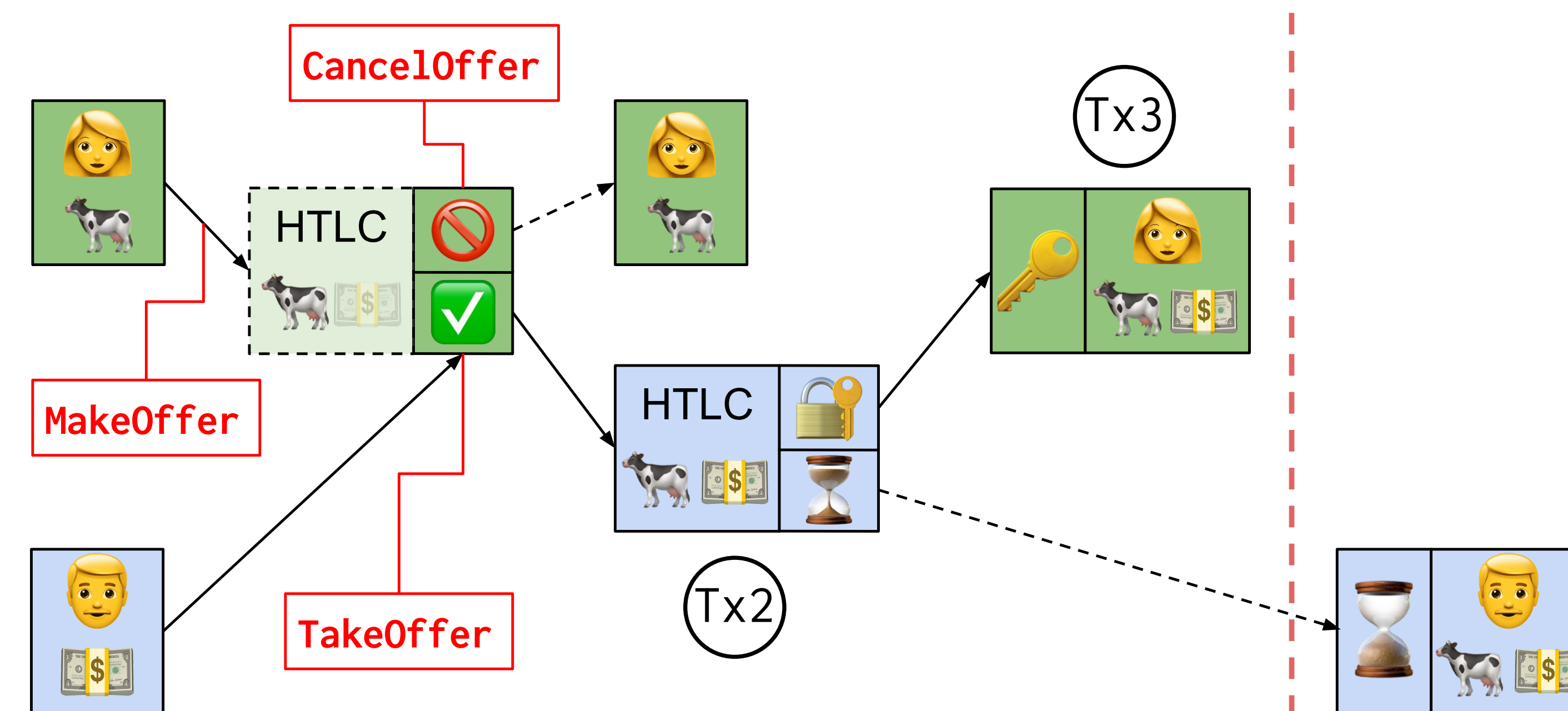
Figure 2: The \beta ledger part of the fair atomic swap protocol
