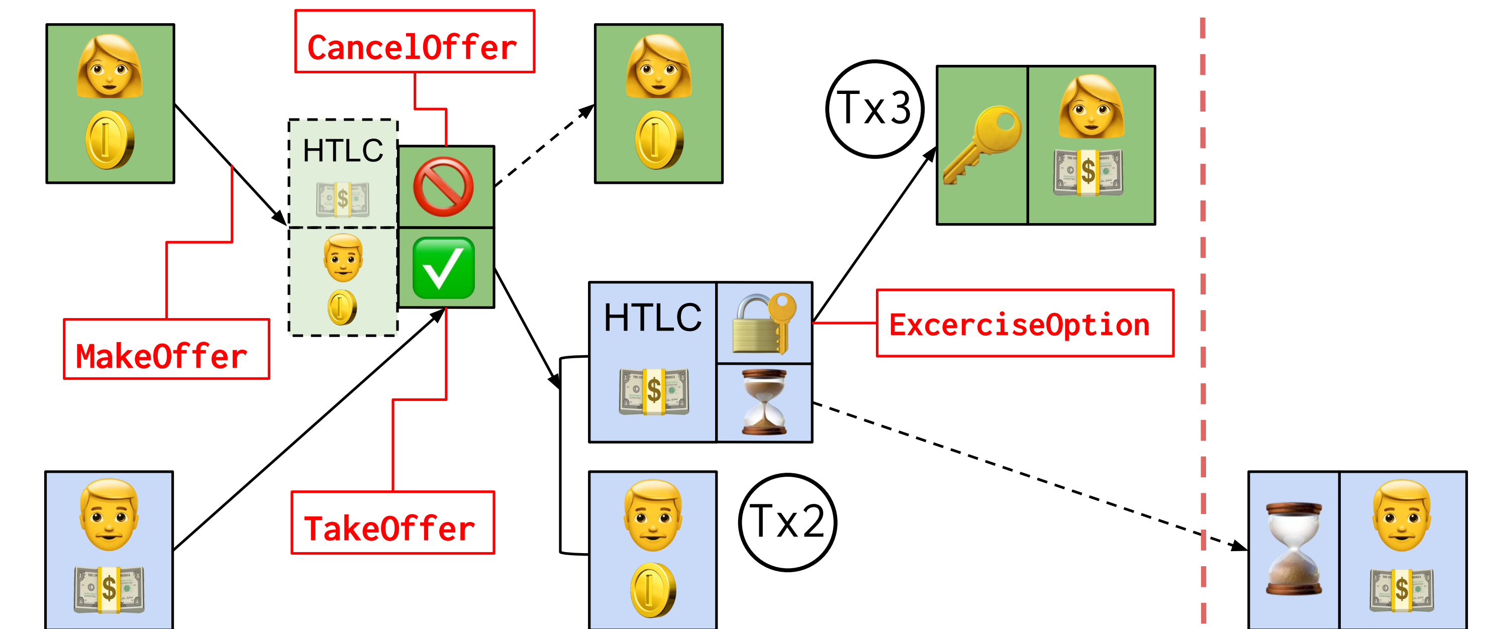
Figure 3: The \beta ledger part of the Fair Option protocol.
